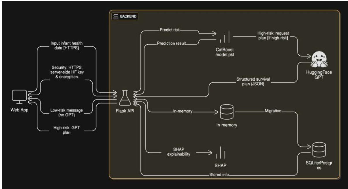
Fig.4.1: System Architecture
